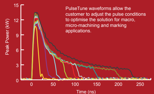
The graph shows a number of waveforms with the option to select from 40 PulseTune characteristics.
